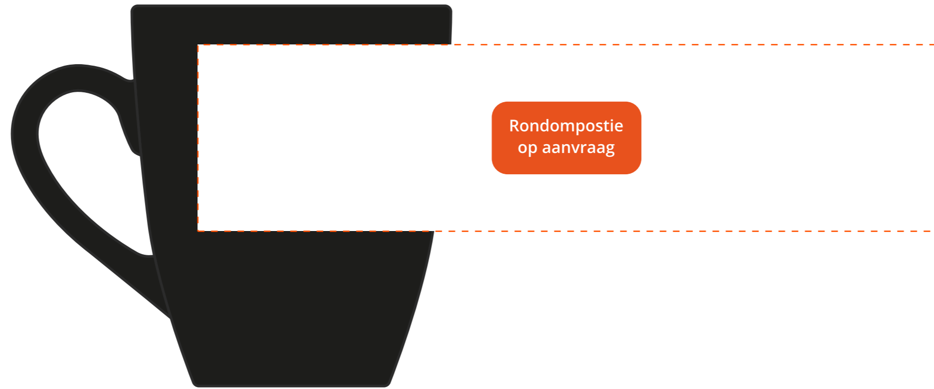
Random
